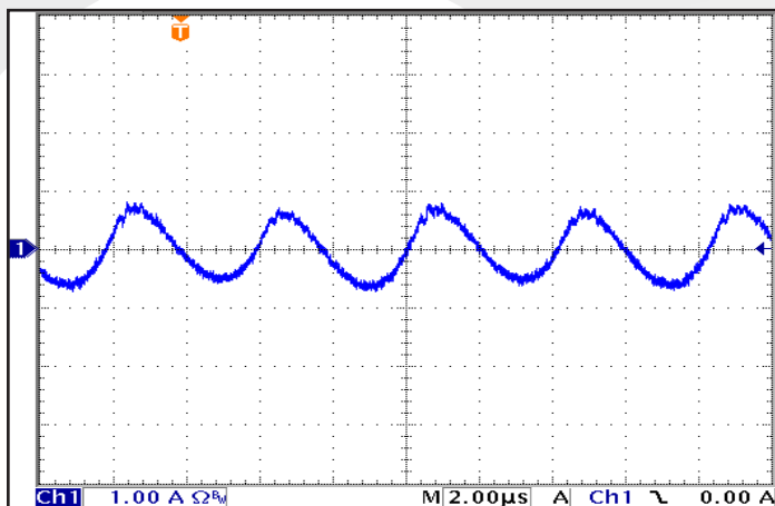
Figure 9: Input Terminal Current Ripple , i_c , at full rated output current and nominal input voltage with 3.3μH source impedance and 470μF electrolytic capacitor (1 A/div). Bandwidth: 20 MHz. Timescale: 2.00μs/div. See Figure 13.
