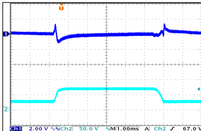
Figure 12: Output Voltage Response to Step-Change in Input Voltage , ( dV/dt = 250 V/ms ). Load capacitance: 100 μF electrolytic output capacitance. Ch 1: V_{out} (2 V/div); Ch 2: V_{in} (50 V/div). Timescale: 1 ms/div.
