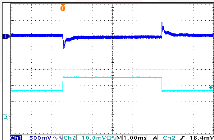
Figure 11: Output Voltage Response to Step-Change in Load Current , (50% -75%-50% of I_{out(max)} ; dI/dt = 5 A/μs ). Load capacitance: 1 μF ceramic and 100 μF electrolytic capacitors. Ch 1: V_{out} (500 mV/div); Ch 2: I_{out} (10 A/div). Timescale: 1.00ms/div.
