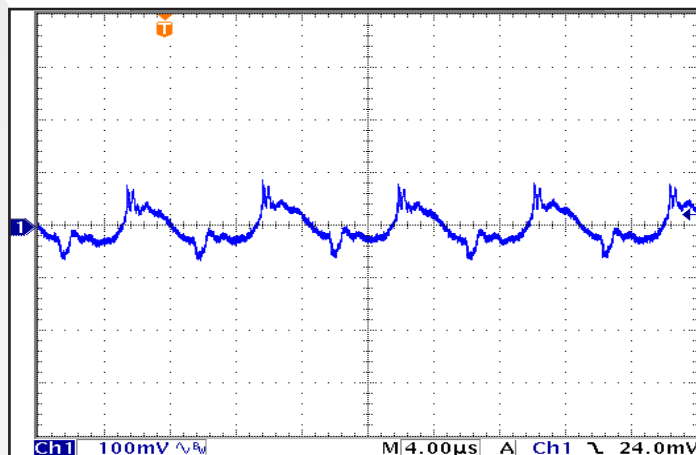
Figure 10: Output Voltage Ripple , V_{out} , at nominal input voltage and rated load current (100 mV/div). Load capacitance: 1 μF ceramic and 100 μF electrolytic capacitors. Bandwidth: 20 MHz. Timescale: 4.00μs/div. See Figure 13.
