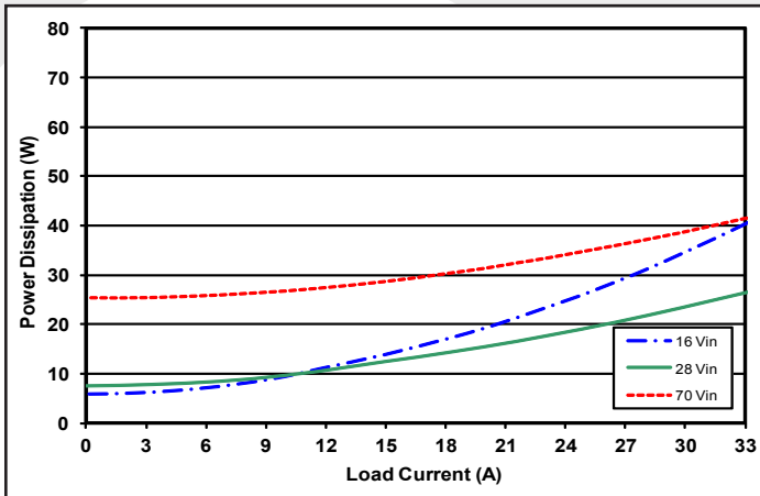
Figure 3: Power Dissipation, at nominal output voltage vs. load current for minimum, nominal, and maximum input voltages at TCASE=25 °C.
